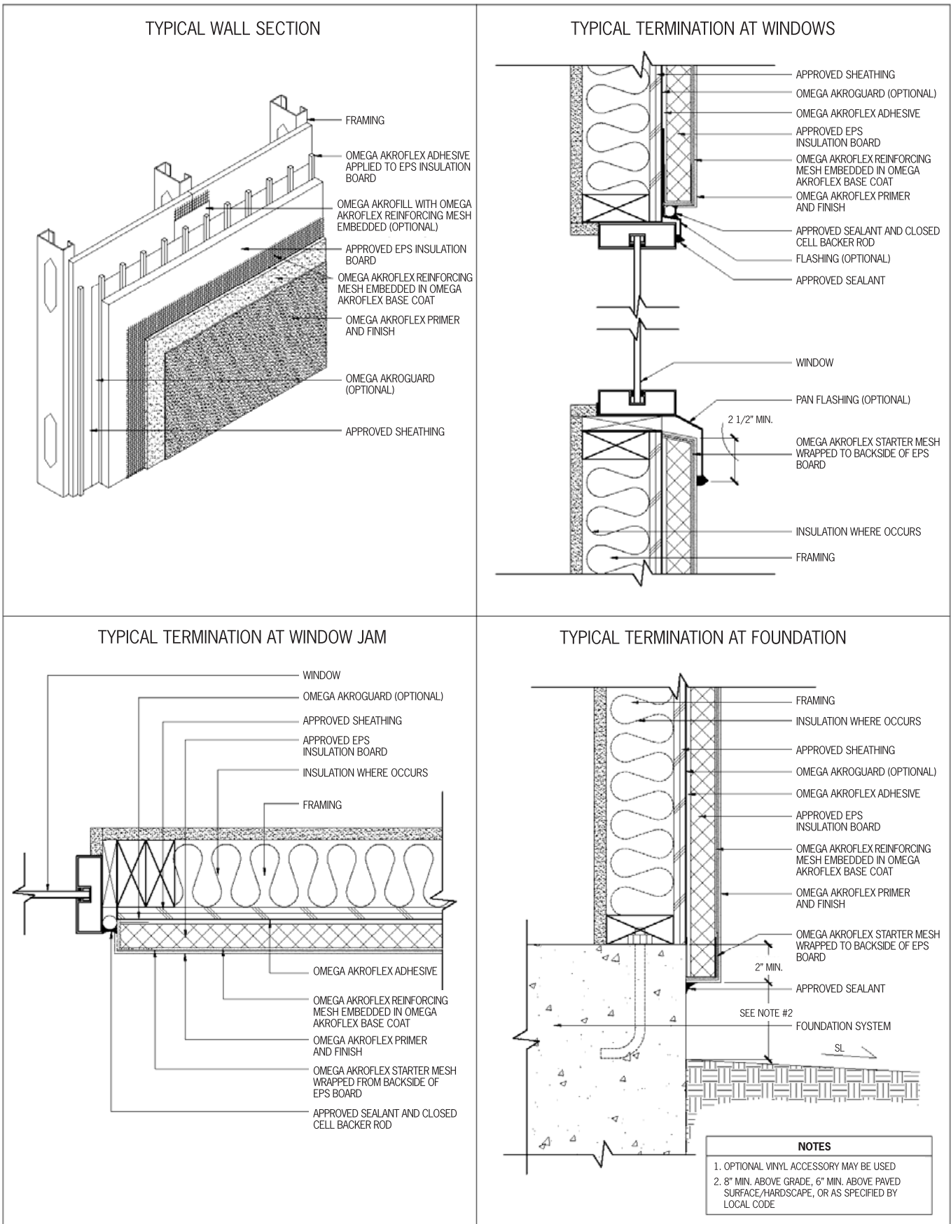
FIGURE 1—TYPICAL INSTALLATION DETAILS
